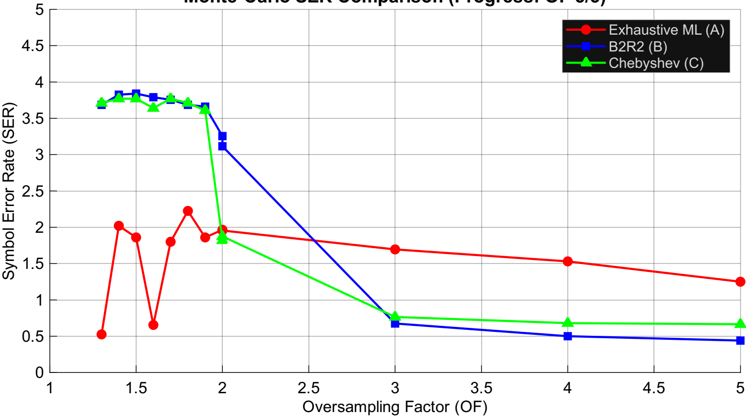
Monte-Carlo SER Comparison (Progress: OF 5/5)
